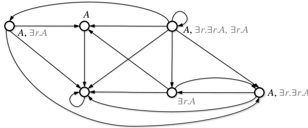
Fig. 3. A finite learning set for an \mathcal{EL}^{\text{lhs}} TBox \{\exists r.\exists r.A \sqsubseteq A\} (all arrows represent r -relations). The figure includes type contents (in grey), as defined in the proof of Theorem 3.
