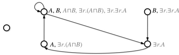
Fig. 2. A finite learning set for an \mathcal{EL}^{\text{rhs}} TBox \{A \sqsubseteq \exists r.(A \sqcap B), B \sqsubseteq \exists r.\exists r.A\} (all arrows represent r -relations). The figure includes type contents (in grey), as defined in the proof of Theorem 2.
