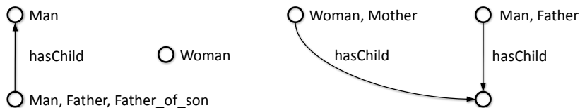
Fig. 1. A sample TIP with an \mathcal{EL} TBox (above, where C \equiv D abbreviates C \sqsubseteq D and D \sqsubseteq C ) and a finite learning set (below).
